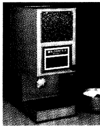
#8730 Integrity® Coffee-Grinder. Heavy gauge steel construction. 115 volts, A.C. 60/hz. 14 1/2" deep, 8 3/4" wide, 22" high (31" high with top open). Complete with cord and plug.
